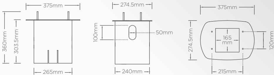
Ground mounting base:
